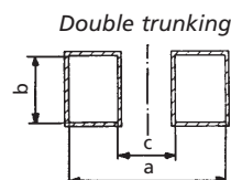
Double trunking
